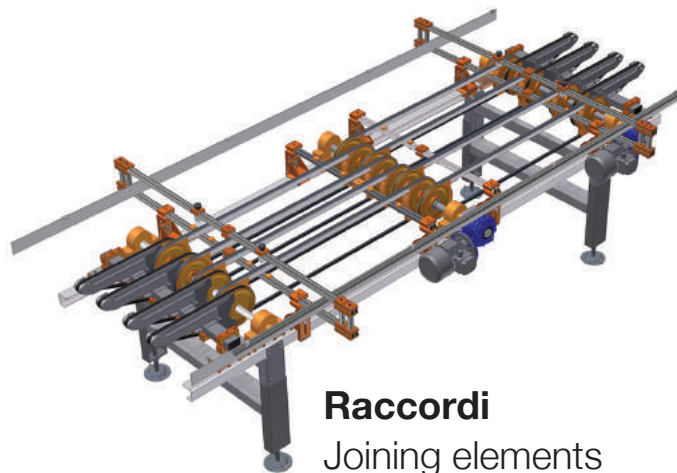
Girelli Turning device
